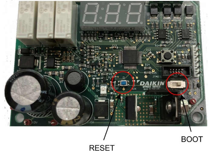
Figure 7: BOOT and RESET Buttons
