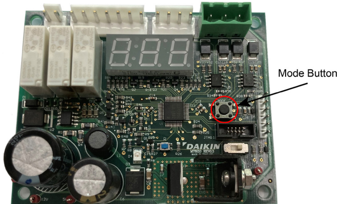
Figure 4: Mode Button Location
