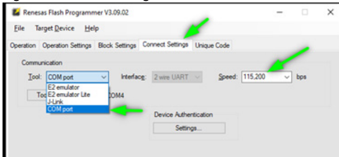
Figure 6: Connect Settings Screen
